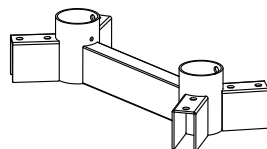
Tube Connector D (X1)
